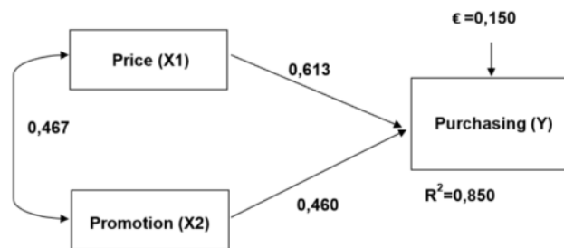
Figure 1. The result of path analysis
