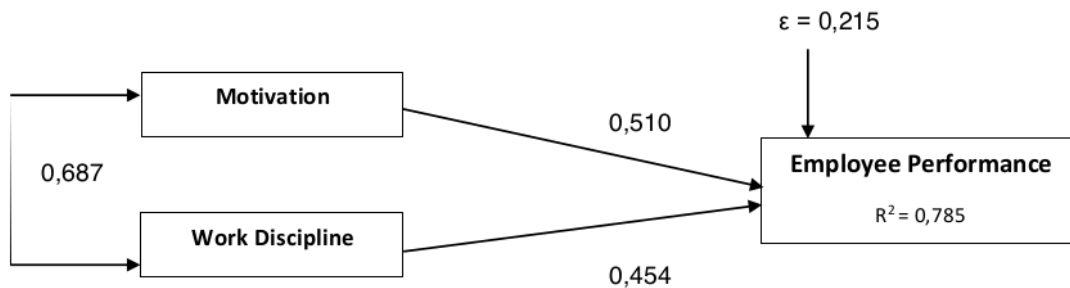
Figure 1. Path Analysis
