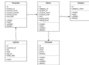
Figure 4. Database Design
