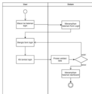
Figure 3. Activity diagram
