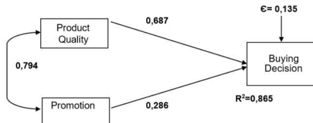
Figure 2. Path Analysis
